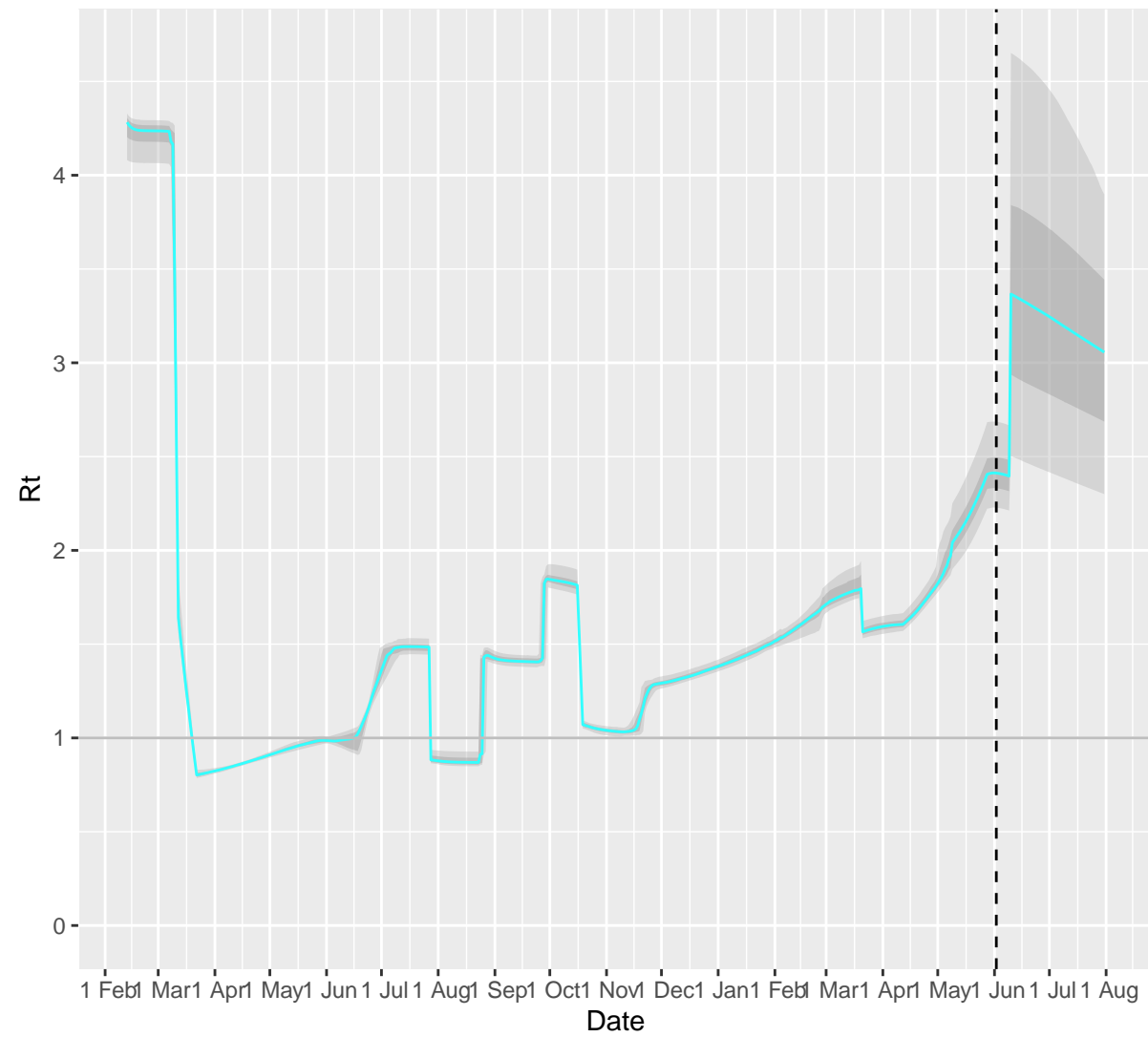
Time-varying reproduction number ( R_t )
