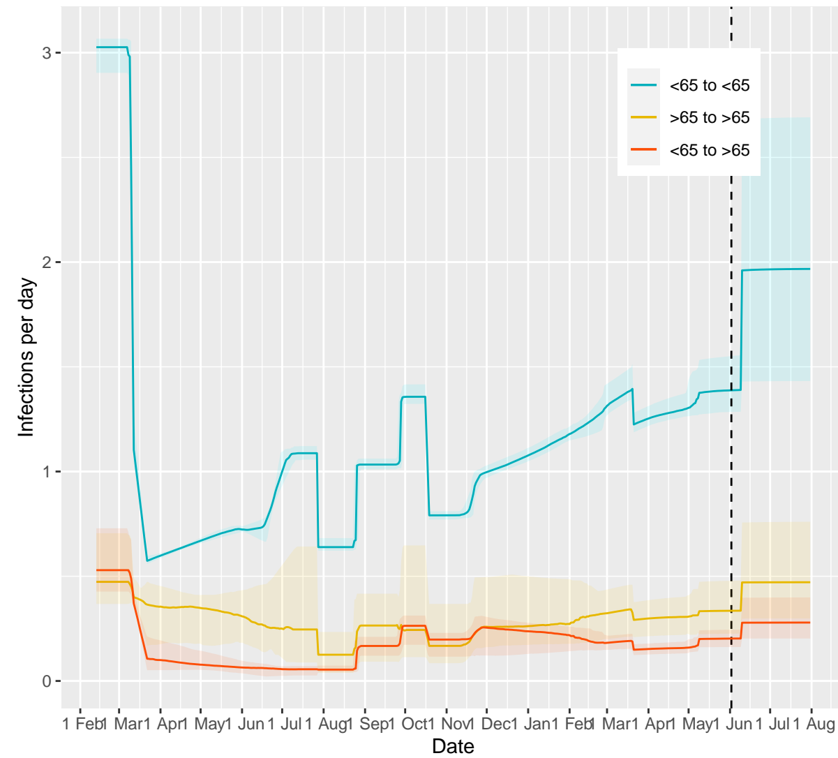
Infections per day per infected individual
